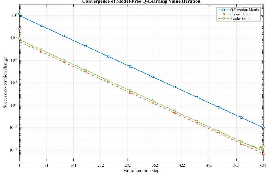
Figure 4.5: Model-Free Q-Learning Value Iteration Convergence
