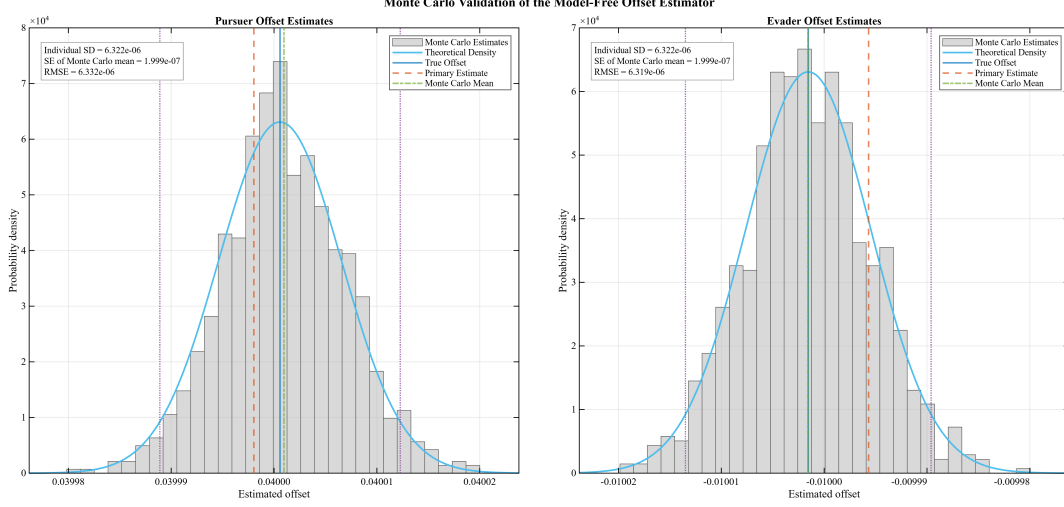
Figure 4.2: Direct Offset-Estimator Monte Carlo Validation for Q-Learning Policy Iteration
