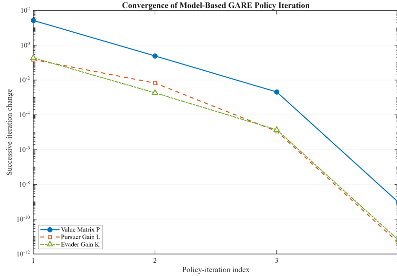
Figure 3.1: Model-Based GARE Policy Iteration Convergence
