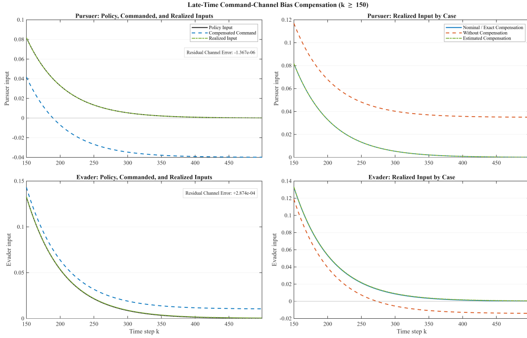
Figure 3.4: GARE Policy Iteration Command Channel Compensation
