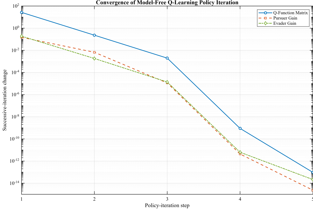
Figure 4.1: Model-Free Q-Learning Policy Iteration Convergence
