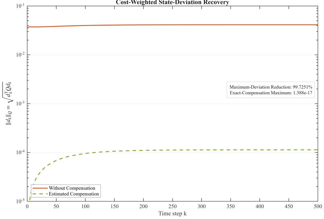
Figure 3.3: GARE Policy Iteration State Deviation Recovery
