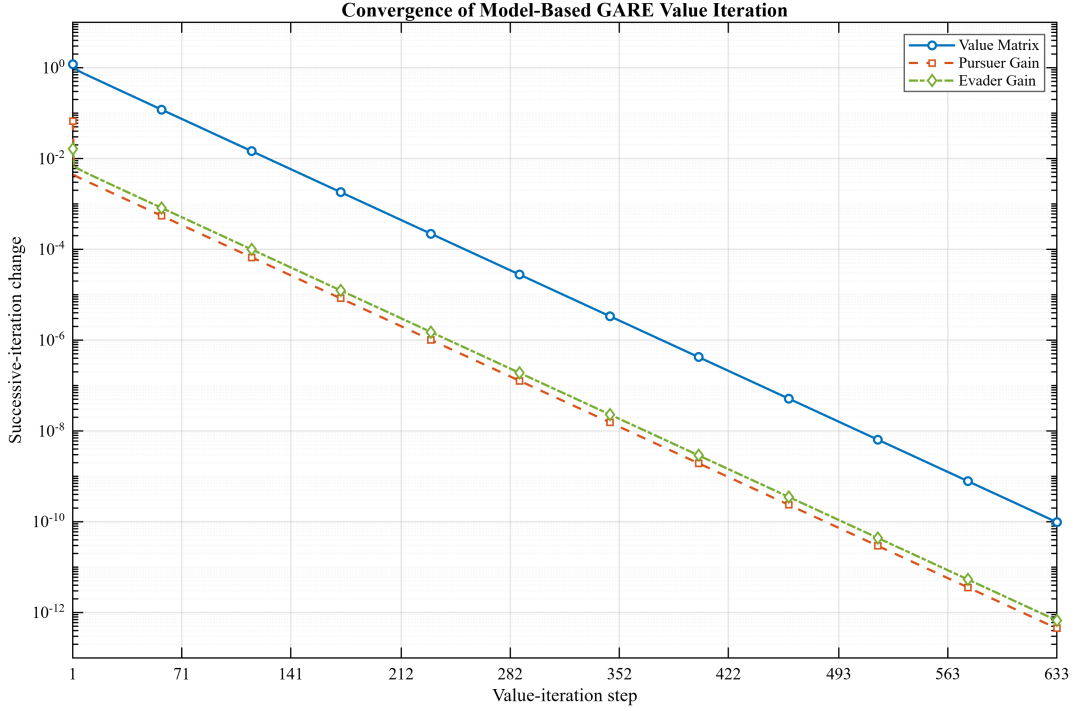
Figure 3.5: Model-Based GARE Value Iteration Convergence
